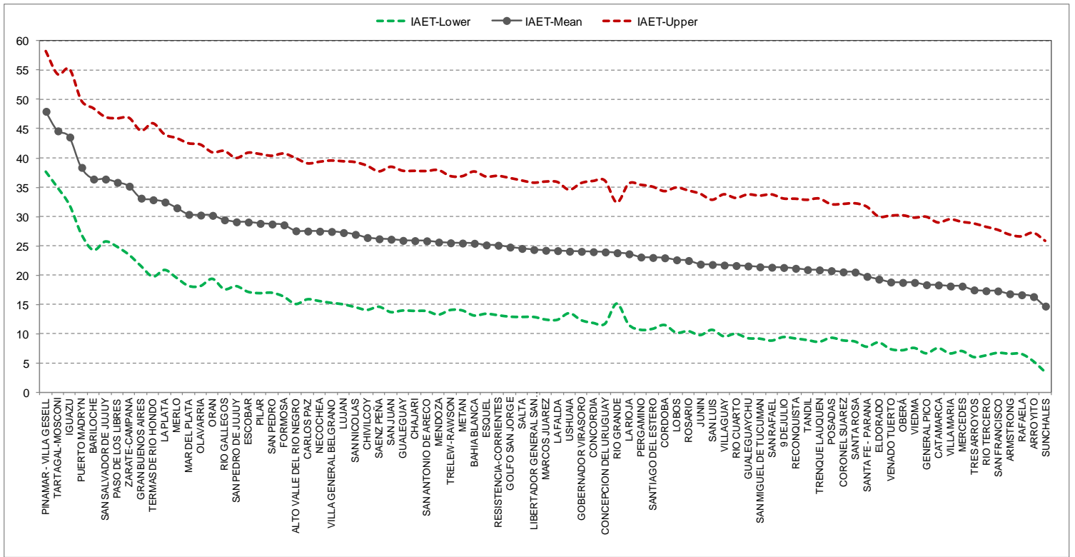
Figure 3: Lower, upper, and average ITEI for LMAs (semester)
